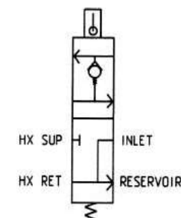
HYDRAULIC SCHEMATIC
